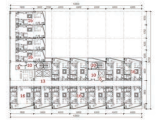
APARTMENT STANDARD PLAN
