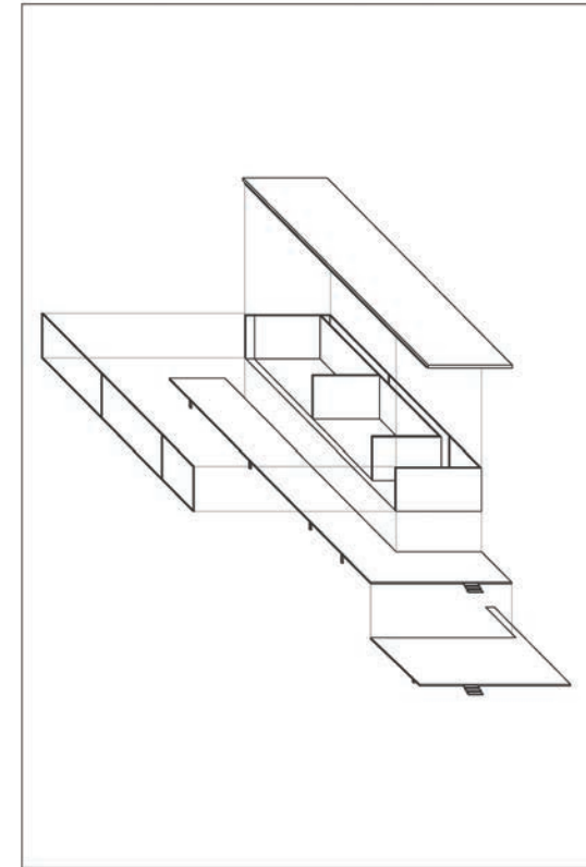
AXONOMETRIC PROJECTION
